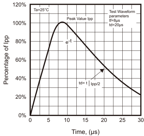
Fig.1 - 8/20μs Peak Pulse Current Waveform Acc. IEC 61000-4-5
